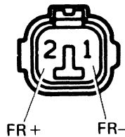
Service Connector (Wire Harness Side)
