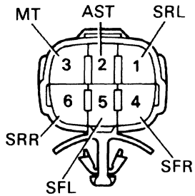
ABS Actuator CONNECTOR A
