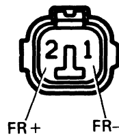
Front Speed Sensor (RH)
