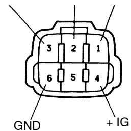
Deceleration Sensor GS1 GS2 GST
